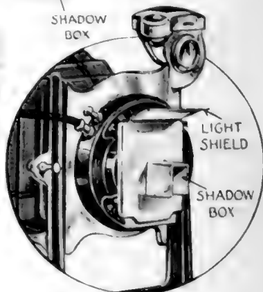
Details of the camera attachment which makes the multiple picture possible
